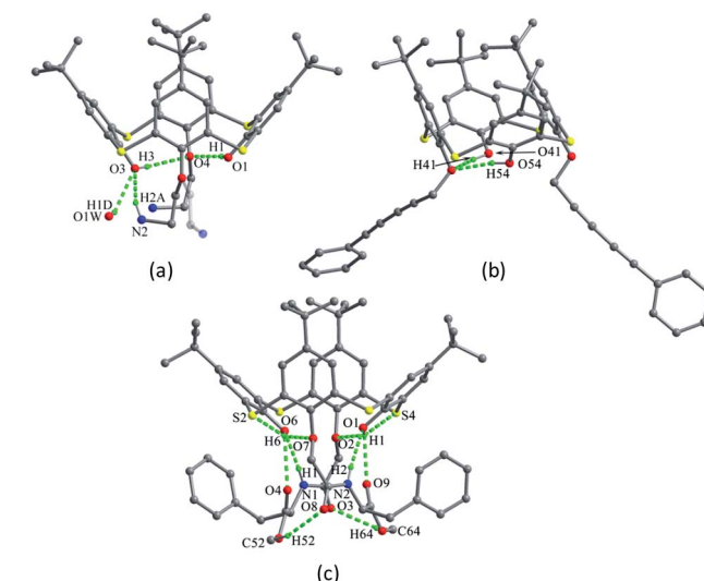
Fig. 21 Crystal structures of 25 (a), 26 (b) and 27 (c), showing H-bonds.
