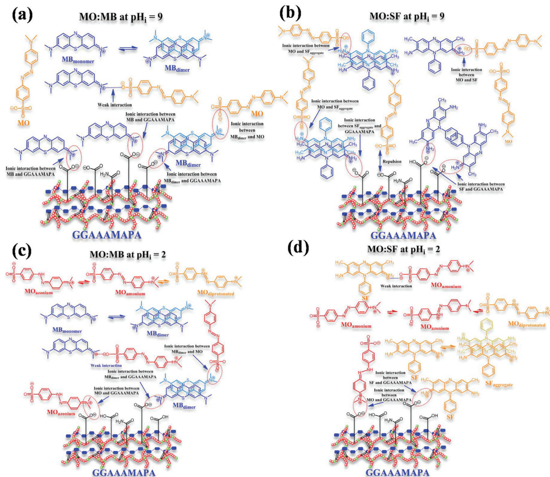
Scheme 5 Synergistic removal of MO and MB at (a) pH_i = 9 and (c) pH_i = 2 and MO and SF at (b) pH_i = 9 and (d) pH_i = 2 .
