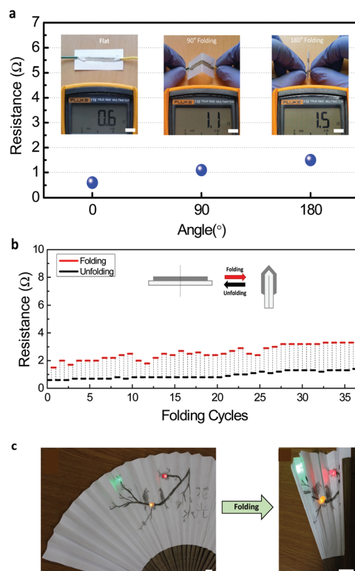
Fig. 4 Electrical and mechanical properties of conductive lines drawn by a hand-written conductive pencil on papers. (a) Resistance measurement of the drawn conductive line (length of 4\text{ cm} and width of 3\text{ mm} ) for unfolded, 90^\circ -folded, and entirely-folded ( 180^\circ ) states. (b) Measured resistance data with multiple folding cycles. Both unfolded (black line), and folded (red line) resistances were measured with the number of folding cycles. (c) Pencil drawing art on a handheld folding fan. The optical images of electronic art on the paper folding fan; drawn oriental painting named 'Mae-hwa'. Red, blue, and green LEDs emitted light with an attached battery in a, unfolded and b, folded states. The electrical current flows through the drawn conductive lines.
