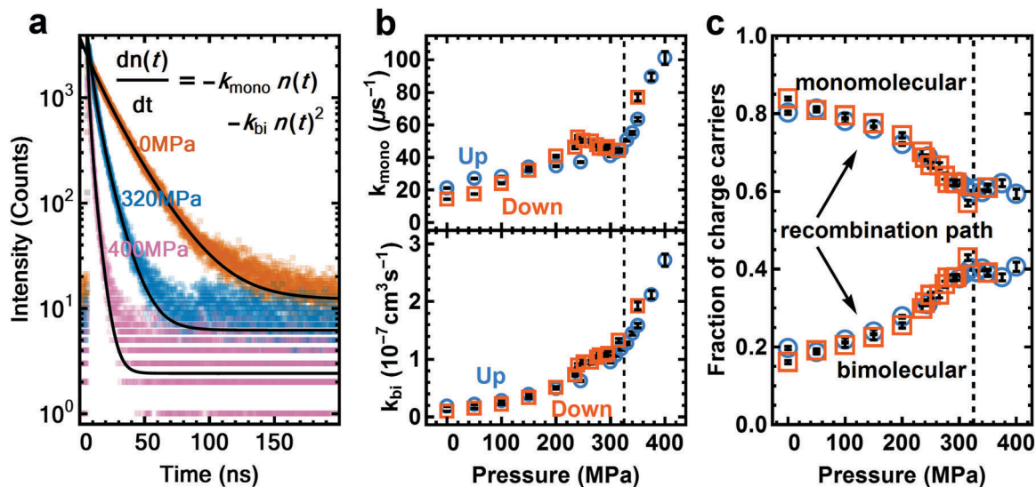
Fig. 2 Time-Resolved Single Photon Counting (TCSPC) data of the PL of a MAPI film under pressure, excited with a 640 nm laser. (a) TCSPC data of 0 MPa, 320 MPa and 400 MPa pressure. The black line shows the fit from the model shown in the inset. (b) Monomolecular (top) and bimolecular (bottom) decay rates of the charge carriers, extracted from the fit. The bimolecular recombination rate (bottom) changes faster with pressure than the monomolecular recombination rate, with both changing slope after the phase transition at 325 MPa (dashed line). Black bars inside symbols represent the error from the fit. (c) Fraction of charge carriers that decayed through the monomolecular channel and bimolecular channel.
