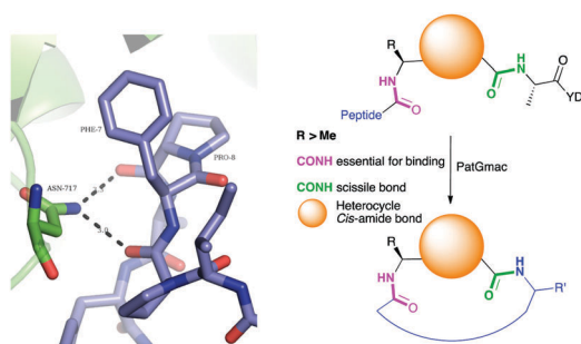
Fig. 2 Left: Hydrogen bonding between the side chain of Asn717 and the carbonyls of substrate. We conclude these hydrogen bonds are critical in substrate recognition and explain the requirement for an L-configured non-glycine residue at position residues 7 of substrate (Phe is shown from PDB 4AKT). Right: PatGmac macrocyclisation substrate requirements: a heterocycle before AYD adopting a cis - or cis -like conformation, a side chain ( R \geq \text{Me} ) preceding the heterocycle. We conclude two substrate carbonyls (coloured green & pink) hydrogen bonded with Asn717 are critical.
