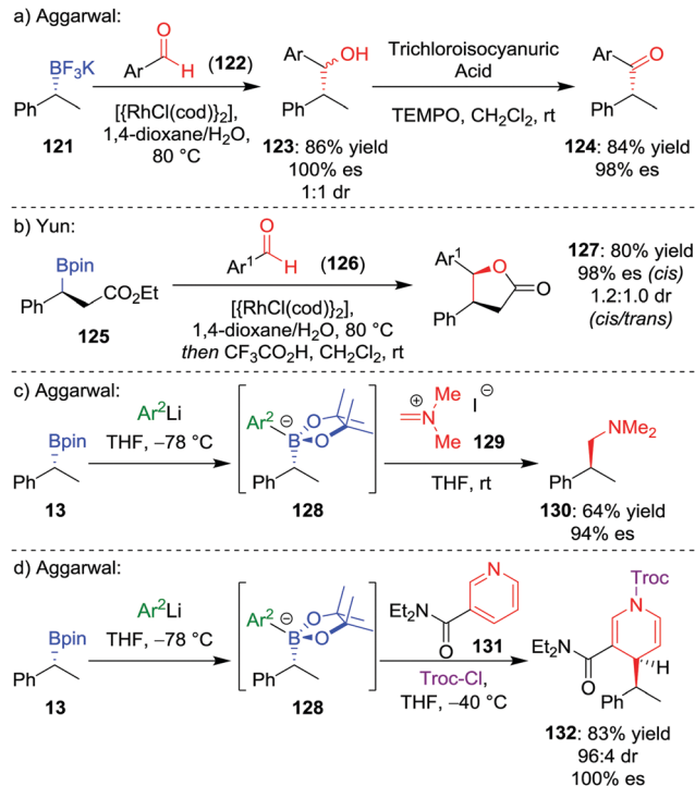
Scheme 18 Additions of trifluoroborate salts and boronate complexes to aldehydes and iminium ions. Ar = p - \text{CF}_3\text{C}_6\text{H}_4 , Ar 1 = p - \text{NO}_2\text{C}_6\text{H}_4 , Ar 2 = 3,5-( \text{CF}_3 ) 2 \text{C}_6\text{H}_3 , Troc-Cl = 2,2,2-trichloroethyl chloroformate.
