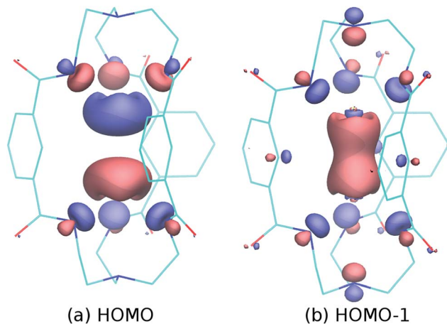
Fig. 2 HOMO (a) and HOMO-1 (b) of the model dianion [Sn_2(mBDCA-5t)]^{2-} based on the crystallographic coordinates of 1 and computed using ORCA 19 at the double-hybrid level of DFT theory 20 B2PLYP-D3/def2-TZVPP with corrections for dispersion 21 and including scalar relativistic effects via the ZORA method. 22
