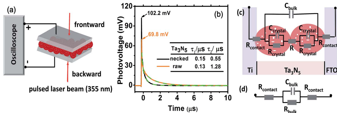
Fig. 5 (a) Schematic setup for TPV test. (b) TPV spectra of raw-Ta 3 N 5 (orange) and necked-Ta 3 N 5 electrode (black) with dual exponential fitted curves (green dashed lines). The inset table shows the lifetimes of the two electrodes, respectively. (c) Equivalent circuit of the device. (d) The simplified circuit of (c). R_{\text{contact}} is the serial resistance at the particle-substrate interfaces; R_{\text{bulk}} is the total resistance in Ta 3 N 5 films including the resistance in Ta 3 N 5 particles ( R_{\text{crystal}} ) and at particle-particle interfaces ( R ); C_{\text{bulk}} is the capacity of the parallel-plate capacitor built by Ti and FTO.
