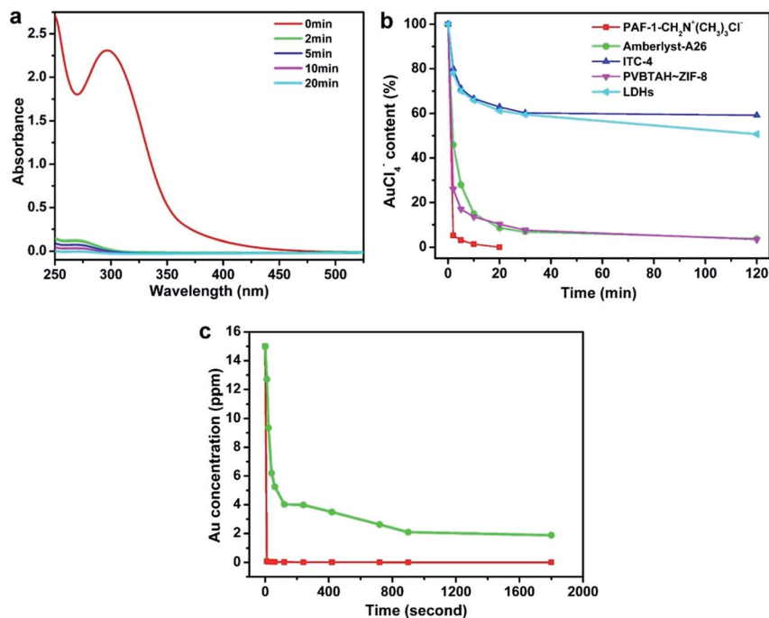
Fig. 2 Kinetics investigation of \text{PAF-1-CH}_2\text{-N}^+(\text{CH}_3)_3\text{Cl}^- . (a) UV-vis spectra of \text{AuCl}_4^- aqueous solution in the presence of \text{PAF-1-CH}_2\text{-N}^+(\text{CH}_3)_3\text{Cl}^- monitored with time. (b) Comparison of the ion exchange performances of \text{PAF-1-CH}_2\text{-N}^+(\text{CH}_3)_3\text{Cl}^- and other ion exchange materials in extracting \text{AuCl}_4^- . (c) \text{Au(CN)}_2^- exchange kinetics of \text{PAF-1-CH}_2\text{-N}^+(\text{CH}_3)_3\text{OH}^- (red) and Amberlyst-A26 (green) with an \text{Au(I)} initial concentration of 15 ppm in \text{KAu(CN)}_2 solution.
