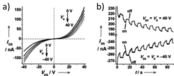
Fig. 10 (a) Output characteristics ( I_{DS} vs. V_{DS} ) of a FET device with nanosheets of 66 . (b) Transient measurement ( V_{DS} = V_G = \pm 40 V) of the transient channel current was recorded with a 40 \text{ mW cm}^{-2} light switching on and off every five seconds in a 90 second period. I_{DS} = drain-source current, V_{DS} = drain-source voltage, V_G = gate voltage (adapted with permission from ref. 123. Copyright 2009, Wiley-VCH Verlag GmbH & Co. KGaA).
