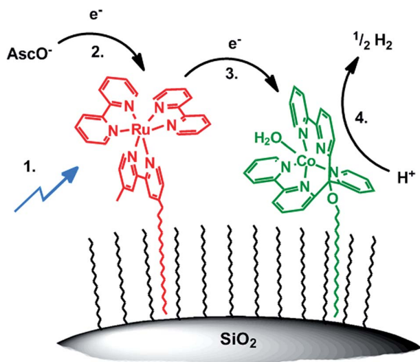
Scheme 4 Proposed reaction mechanism of photocatalytic H 2 production on hydrophobic silica: (1) photoexcitation of 1 → 1* ; (2) reductive quenching of 1* → 1 - ; (3) electron transfer 1 - → 3 ; (4) H + reduction by 3 - .
