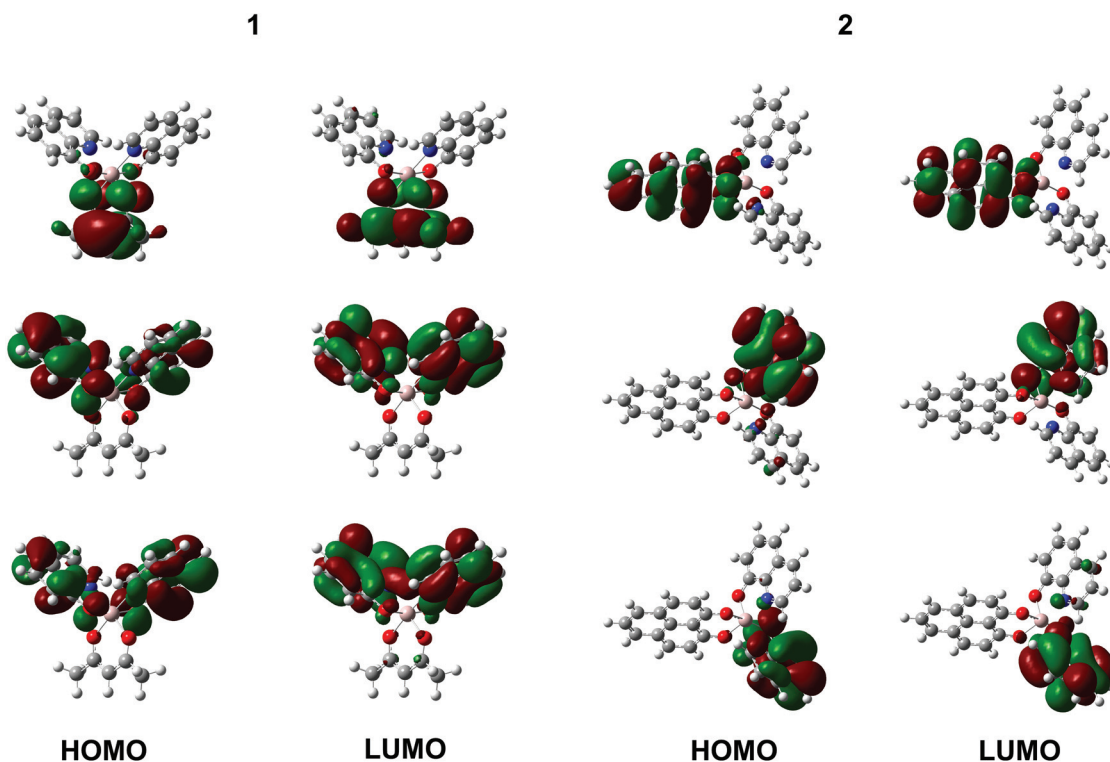
Fig. 5 Electron density of the three degenerate HOMO and LUMO orbitals of 1 (left) and 2 (right), as calculated with DFT. The electron density iso-surfaces with positive and negative values are represented by the green and red bubbles, respectively.
