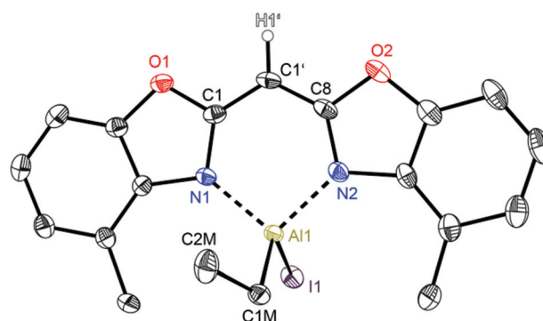
Fig. 9 Molecular structure of [\text{IEtAl}\{(\text{4-MeNCOC}_6\text{H}_3)_2\text{CH}\}] ( 7 ). Anisotropic displacement parameters are depicted at the 50% probability level. C–H hydrogen atoms are omitted for clarity except for the one at the bridging CH group. Structural data are given in Tables 1–3.
