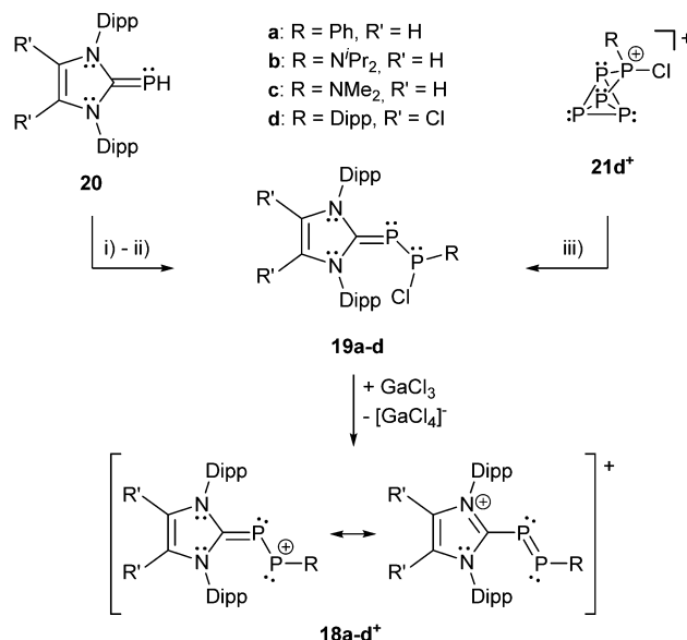
Scheme 7 Two different approaches for the synthesis of NHC stabilized chlorodiphosphenes 19a-d comprising bonding motif B. For 19a,b : (i) +R'PCl_2 , +DABCO , -DABCO\cdot HCl ; for 19c : (ii) +2PCl(NMe_2)_2 , +DABCO , -DABCO\cdot HCl , -P(NMe_2)_3 ; for 19d : (iii) +3 1,3-bis(2,6-diisopropylphenyl)-4,5-dichloro-imidazole-2-ylidene, -5^+ . Subsequent chloride abstraction yields polarized cationic diphosphenes 18a-d + . Only two resonance structures that indicate the polarization of 18a-d + are shown.
