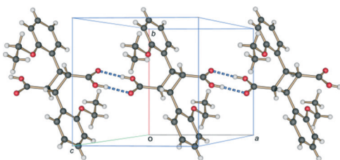
Fig. 16 Hydrogen bonded carboxylic acid dimer chain, running parallel to the a axis, present in the crystal structure of 2,2'-diethoxy- \alpha -truxillic acid (CSD recode XOSKEV ) – the final photoproduct at the end of stage 2.
