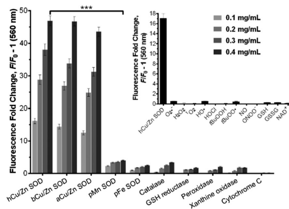
Fig. 2 Fluorogenic response of SODO upon binding to different proteins (at 0.1, 0.2, 0.3 and 0.4 mg mL -1 ) and metabolites (inset, ROS & RNS: 100 µM) in 20 mM Tris-HCl buffer (pH = 7.4). \lambda_{exc} : 460 nm, \lambda_{em} : 560 nm. Values are represented as means and error bars as standard deviations ( n = 3 ), *** for p < 0.001 .
