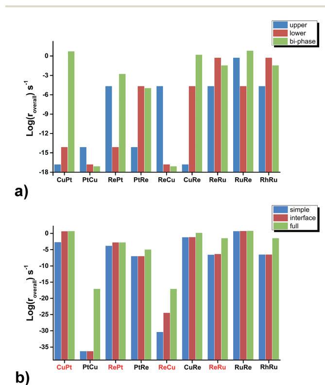
Fig. 3 Activity ( \text{log}(r_{\text{overall}}) ) comparisons of nine bi-phase surfaces among (a) those from the upper phase, lower phase and bi-phase surfaces, respectively, (b) the simple, interface and full kinetic models, where the reactive-noble bi-phase surfaces are highlighted in red.
