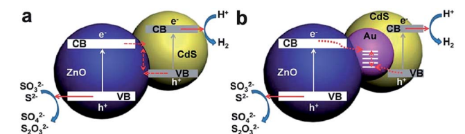
Fig. 29 Schematic presentation of: (a) the direct Z-scheme charge-carrier transfer process in CdS–ZnO and (b) the vectorial Z-scheme charge-carrier transfer process in CdS–Au–ZnO (reprinted with permission from ref. 344; Copyright 2013 @ Royal Society of Chemistry).
