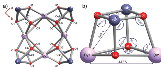
Fig. 2 (a) The \text{Dy}(\text{III}) vertex-sharing arrangement of four \text{Dy}_2\text{Cu}_2 cubanes to constitute a \text{Dy}_4\text{Cu}_8 dodecahedron architecture, viewed along c-axis; (b) intermetallic distances and bond angles spanned at different vertices of each of the four \text{Dy}_2\text{Cu}_2 constituent cubanes of the symmetric heterometallic core.
