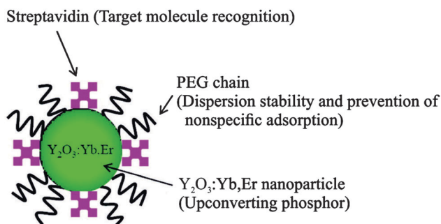
Fig. 16 Scheme of UCNPs coated by PEG-PAA and streptavidin by ligand exchange reaction. The polymer increases the dispersion stability and prevents non-specific binding, while streptavidin serves as a binding site for target molecules. Reprinted with permission from ref. 33. Copyright © 2008, American Chemical Society.
