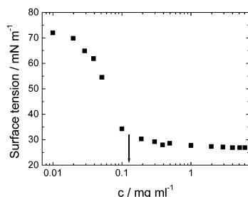
Fig. 5 Surface tension versus concentration used to determine the cmc for viscosin (shown by arrow). Redrawn from ref. 23a.
