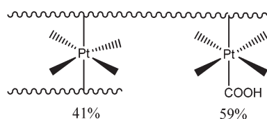
Scheme 3 Conjugation of Pt(IV) [(\text{COOH})_2] as a crosslinker for the amine bearing monomers.
