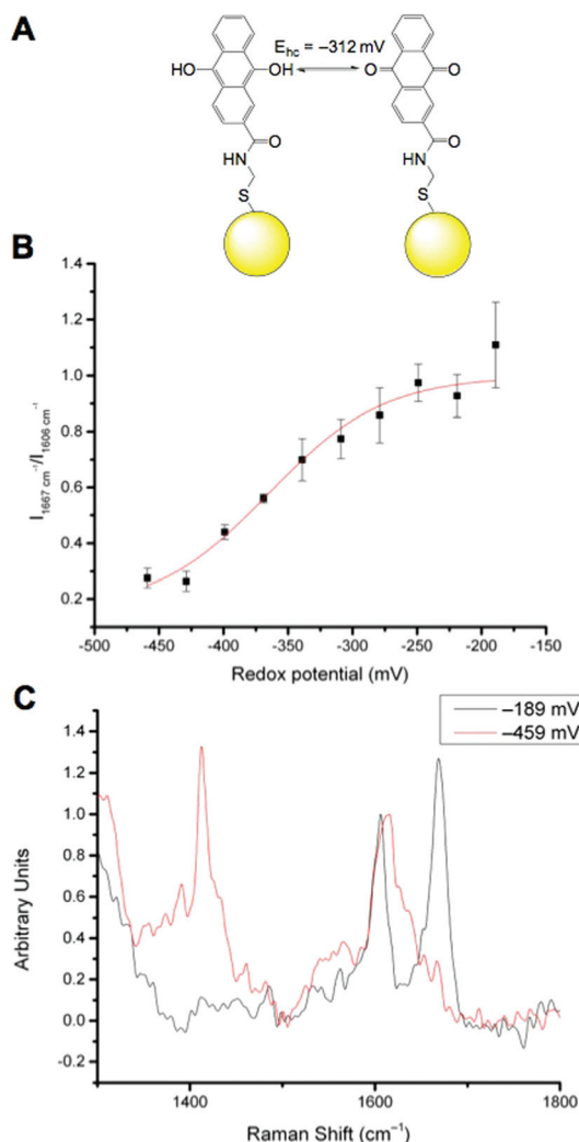
Fig. 2 AQ-NP nanosensor. (A): Equilibrium between oxidised and reduced AQ attached to a gold NP (yellow sphere, not to scale). (B): Calibration curve for AQ-NP nanosensors ( R^2 = 0.96855 ). (C): Representative spectra of fully oxidised ( -189 mV) and fully reduced ( -459 mV) AQ-NPs.
