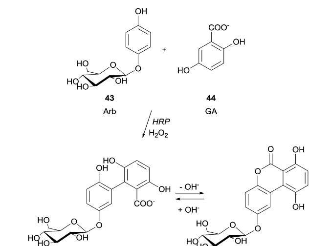
Scheme 13 Coupling of 4'-hydroxyphenyl- \beta -D-glucoside (arbutin, Arb) ( 43 ) with 2,5-dihydroxybenzoic acid sodium salt (gentisate, GA) ( 44 ).
