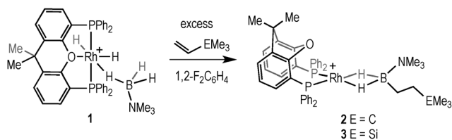
Scheme 2 Formation of 2 (E = C) and 3 (E = Si). [\text{BAR}^F_4]^- anions not shown.
