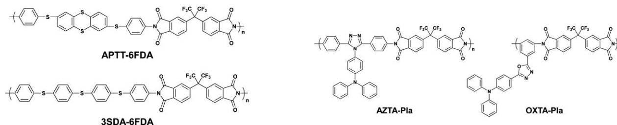
Scheme 5 Chemical structures of AZTA-Pla and OXTA-Pla.
