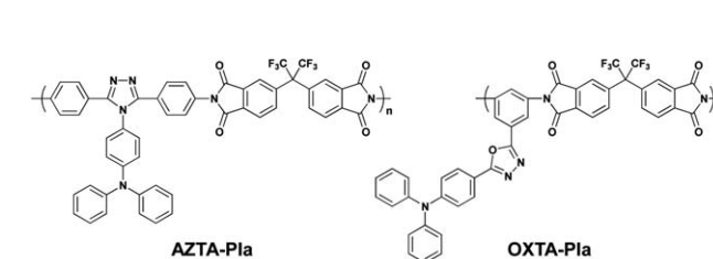
Scheme 5 Chemical structures of AZTA-Pla and OXTA-Pla.
