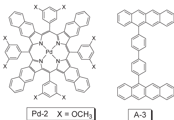
Fig. 10 Molecular structures of palladium complex Pd-2 and the triplet acceptor A-3 used for the upconversion. The compounds are from ref. 31.
