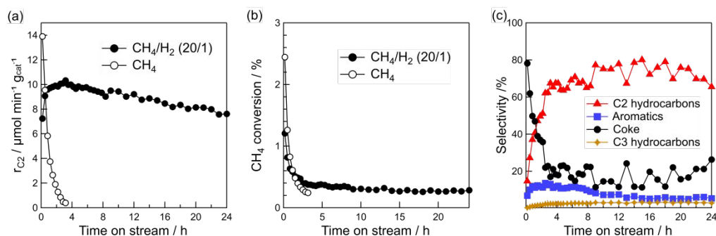
Fig. 6 Time course of (a) formation rate of C2 hydrocarbons, (b) methane conversion, and (c) product selectivity for DCM reaction. Catalyst: Pt(1)/Al 2 O 3 , T: 600 °C, flow rate: 20 (CH 4 ) and 20+1 (CH 4 +H 2 ) mL min -1 , and catalyst mass: 0.10 g.
