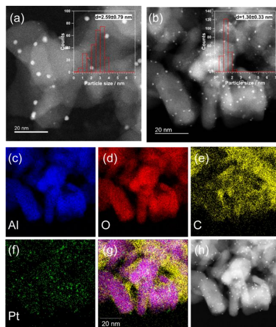
Fig. 2 HAADF-STEM images and particle size distribution of (a) fresh and (b) spent Pt(1)/Al 2 O 3 . EDX mapping images for (c) Al, (d) O, (e) C, (f) Pt, (g) overlay of (c–f), and (h) HAADF-STEM image of the spent catalyst. Spent catalyst: DCM was performed on Pt(1)/Al 2 O 3 for 5h under CH 4 /H 2 (20/1).
