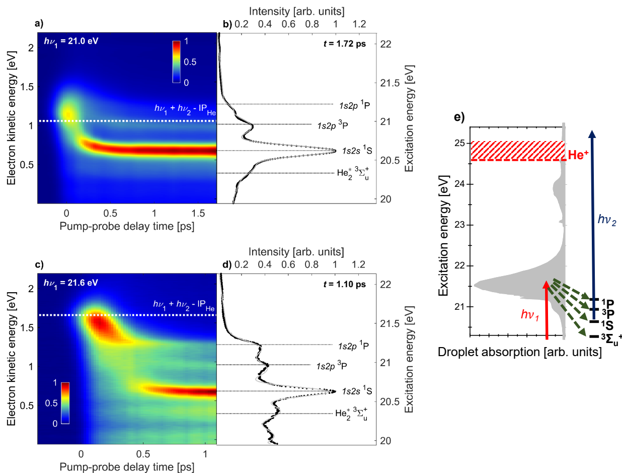
Fig. 2 Time-resolved photoelectron spectra of He droplets measured with XUV-pump and UV-probe pulses at photon energies h\nu_1 = 21.0 eV [a) and b)] and h\nu_1 = 21.6 eV [c) and d)]. The maps [a) and c)] are composed of 28 and 31 spectra at different pump-probe delays, respectively. The white dashed lines indicate the expected electron energies for direct 1+1' photoionization. Panels b) and d) show the electron spectra at fixed delays of 1.7 ps and 1.1 ps, respectively. The black horizontal lines indicate the expected electron energies for photoionization of specific excited states of quasifree \text{He}^* atoms and \text{He}_2^* excimers. The gray line is the multi-Gaussian fit to the experimental spectra. See the main text for additional details. Panel e) shows the He droplet absorption spectrum from Joppien et al. 9 and the energy levels populated in the course of relaxation. The red and blue arrows represent the pump and probe pulses, respectively, and the green arrows represent the relaxation channels.
