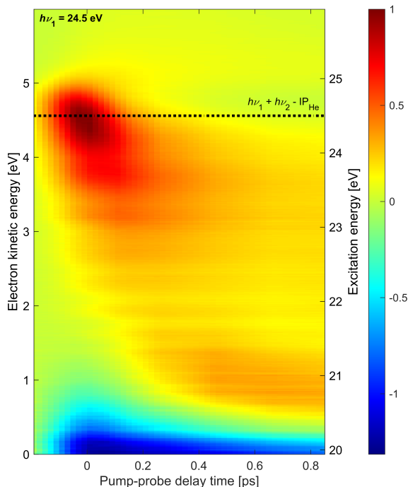
Fig. 4 Time-resolved photoelectron spectra recorded at h\nu_1 = 24.5 eV composed of 13 spectra at different pump-probe delays. The dashed line indicates the expected electron energy for direct 1+1' photoionization.
