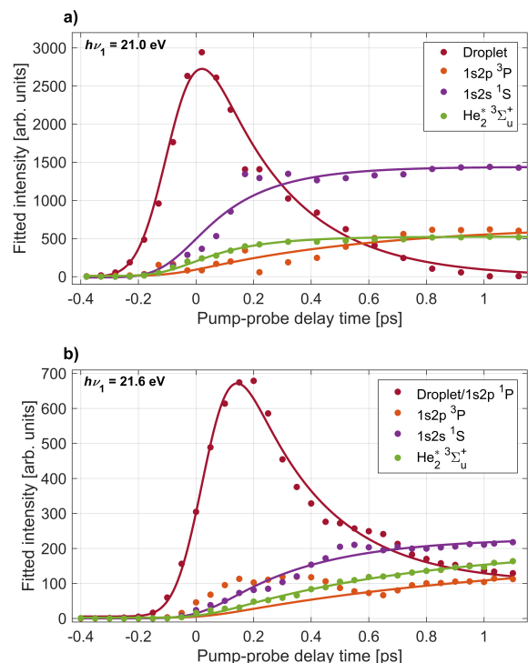
Fig. 3 Results of peak fits to the delay-dependent electron spectra recorded at pump photon energies h\nu_1 = 21.0 eV [panel a)] and h\nu_2 = 21.6 eV [panel b)]. Shown are the integrated areas of Gaussian peaks fitted to the individual components in the electron spectra, labeled in Fig. 2. The largest ‘Droplet’ peak corresponds to the bright feature dominating the electron spectra around zero delay. The smooth lines depict fits of the data with Eqs. (3) and (4) from which characteristic time constants for the appearance of the individual components are inferred.
