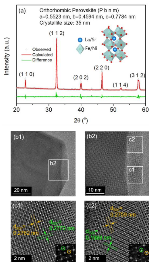
Fig. 1. (a) XRD pattern of La_{0.7}Sr_{0.2}Ni_{0.2}Fe_{0.8}O_3 perovskite (LSNF) powder at room temperature and Rietveld refinement of the XRD pattern, (b) TEM images of LSNF at room temperature, (c) enlarged TEM images of the specified area from (b) with lattice fringes and inverse fast Fourier transform (IFFT) of the selected area.
