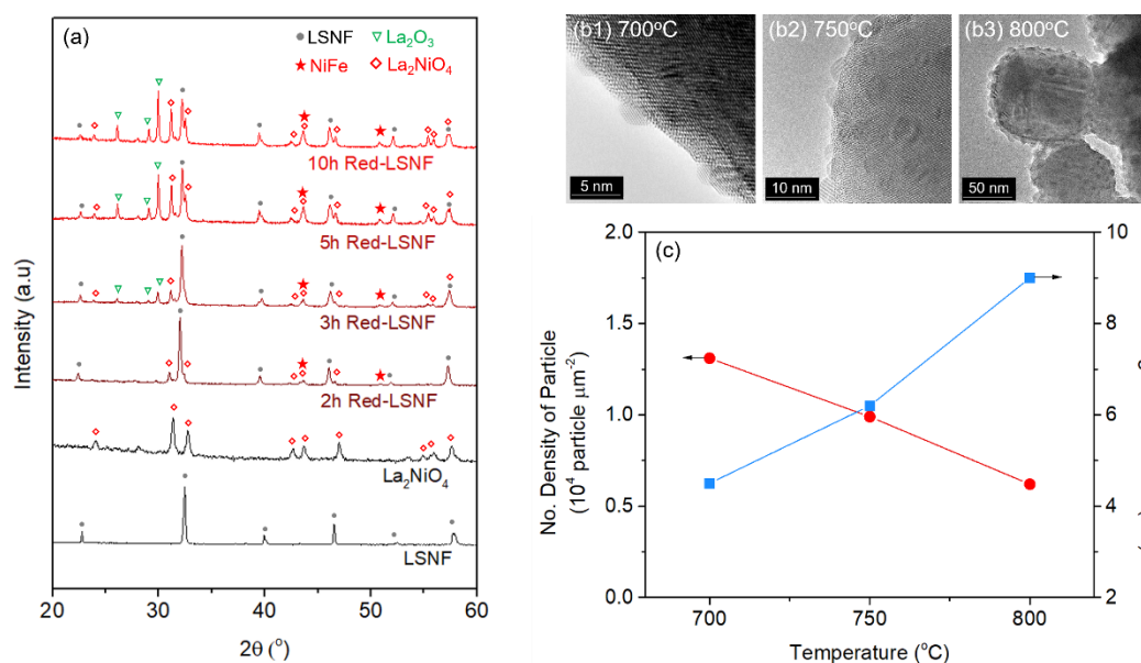
Fig. 4. (a) XRD patterns of LSNF, La 2 NiO 4 , and LSNF treated with 5% H 2 /N 2 atmosphere at 800°C with different time duration, (b) in-situ TEM images of LSNF powders under 1 mbar of H 2 atmosphere at 700°C, 750°C, and 800°C, (c) the number densities and average particles sizes of the exsolved nanoparticles on the LSNF surface at 700°C, 750°C, and 800°C.
