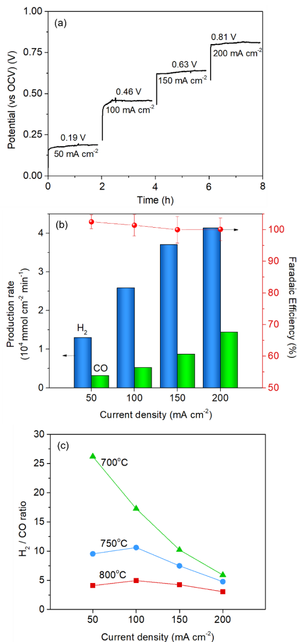
Fig. 11. (a) Current-voltage relationship of the Red-LSNF cell, (b) normalized production rate of H 2 and CO with Faradaic efficiency for co-electrolysis of H 2 O/CO 2 at 800°C at different current densities, (c) H 2 /CO ratio at different temperatures and at different current densities.
