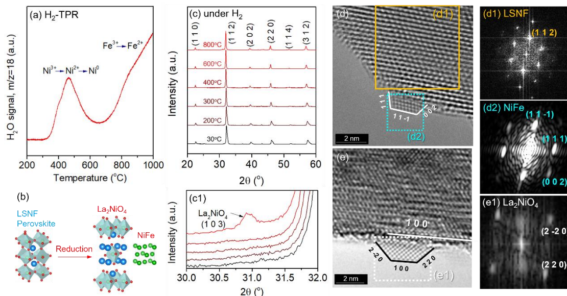
Fig. 3. (a) Temperature-programmed reduction profile of LSNF powders under 30 ccm of 5% H 2 /N 2 with a 20°C min -1 ramp rate (b) illustration of the formation of zerovalent Ni and La 2 NiO 4 in a Ruddlesden-Popper phase during the reduction and exsolution process, (c) in-situ XRD patterns of LSNF powders under 5% H 2 /N 2 atmosphere at various temperatures heating from 30°C and 800°C, (c1) the (1 0 3) diffraction peak of La 2 NiO 4 in an enlarged scale, (d) in-situ TEM image of LSNF under 1 mbar of H 2 atmosphere at 500°C with an exsolved NiFe nanoparticle, (d1) IFFT of the area confined for LSNF from (d), (d2) IFFT of the area selected for the exsolved NiFe nanoparticle from (d), (e) in-situ TEM image of LSNF powder under 1 mbar of H 2 at 700°C with an exsolved La 2 NiO 4 nanoparticles, (e1) IFFT of the area confined for the La 2 NiO 4 nanoparticle from (e).
