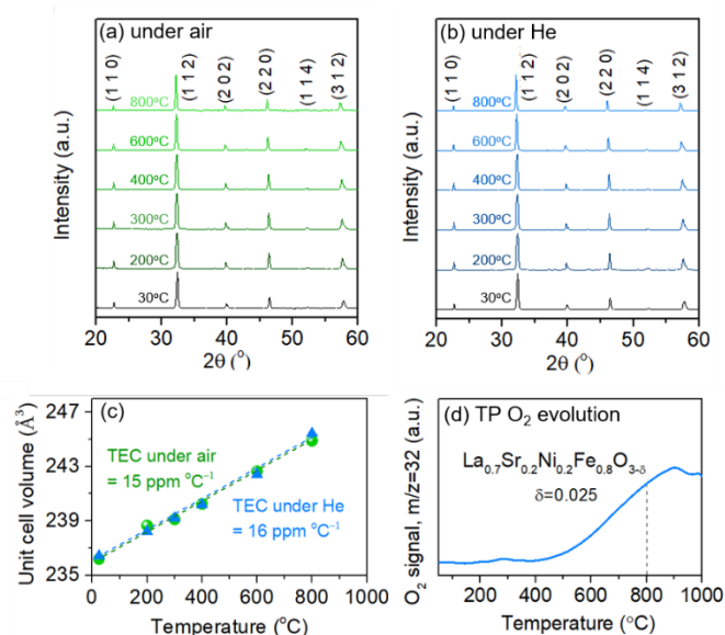
Fig. 2. In-situ XRD patterns of LSNF powders at various temperatures from 30°C to 800°C under (a) air and (b) helium environment, (c) Thermal expansion coefficient of the LSNF powders under air and helium environment, (d) Temperature-programmed O 2 evolution of the LSNF powder under helium environment. \delta represents the created oxygen vacancy per formula unit of LSNF from room temperature to 800°C.
