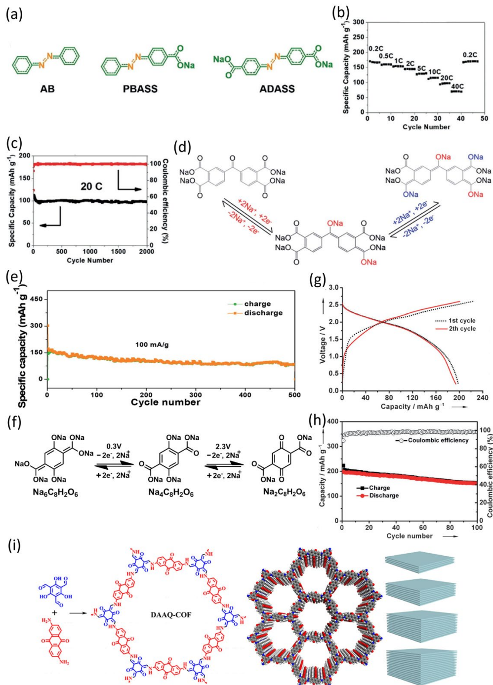
Figure 6. (a) Molecular structure of AB, PBASS, and ADASS. (b) Rate performance at various C-rates. (c) De-sodiation capacity and Coulombic efficiency versus cycle number at 20C. Reproduced with permission. 76 Copyright 2018 Wiley-VCH Verlag GmbH & Co. KGaA. (d) The proposed mechanism of Na ion insertion/extraction into/from the molecular structure of SCID.
