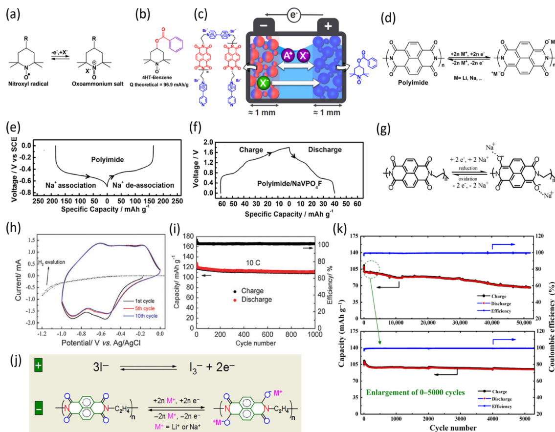
Figure 8. (a) Schematic of the redox reaction of TEMPO derivatives, (b) Structure of TEMPO derivative, 4HT-benzene. (c) Schematic of 4HT-benzene|DNVBr full cell in 8 M NaClO 4 . Reproduced with permission. 88 Copyright 2019 American Chemical Society. (d) Reaction mechanism of NTCDA. Discharge-charge curves of (e) NTDCA electrode and (f) NTDCA|NaVPO 4 F full cell in 5 M NaNO 3 at 50 \text{ mA g}^{-1} . Reproduced with permission. 90 Copyright
