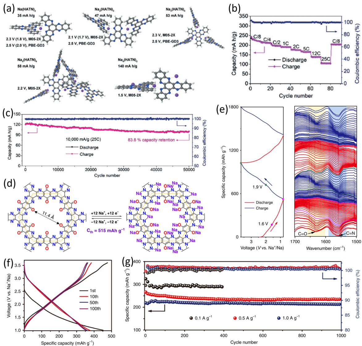
Figure 3. (a) Optimized geometries and insertion potentials vs. Na/Na + of the Na m (HATN) n complexes surrounded by implicit solvent from DFT calculations using M05-2X/6–31+G(d,p) and PBE-GD3/6–31+G(d,p) DFT calculations. (b) Rate capability at various current densities from C/8 to 25 C. (c) Long-term cycling performance of PHATN under the current densities of 10 A g -1 (25C) for 50,000 cycles. Reproduced with permission. 71 Copyright 2019 Wiley-VCH Verlag
