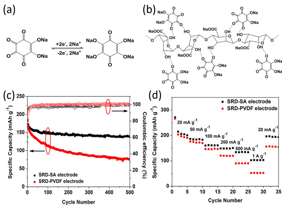
Figure 4. (a) The sodiation-desodiation mechanism for SRD. (b) Schematic illustration of hydrogen bonding between SRD and SA. (c) Cycle life of the SRD-PVDF and SRD-SA electrodes at a current density of 50\text{ mA g}^{-1} . (d) Rate capability of the SRD-SA and SRD-PVDF electrodes. Reproduced with permission. 59 Copyright 2017 Elsevier Inc.
