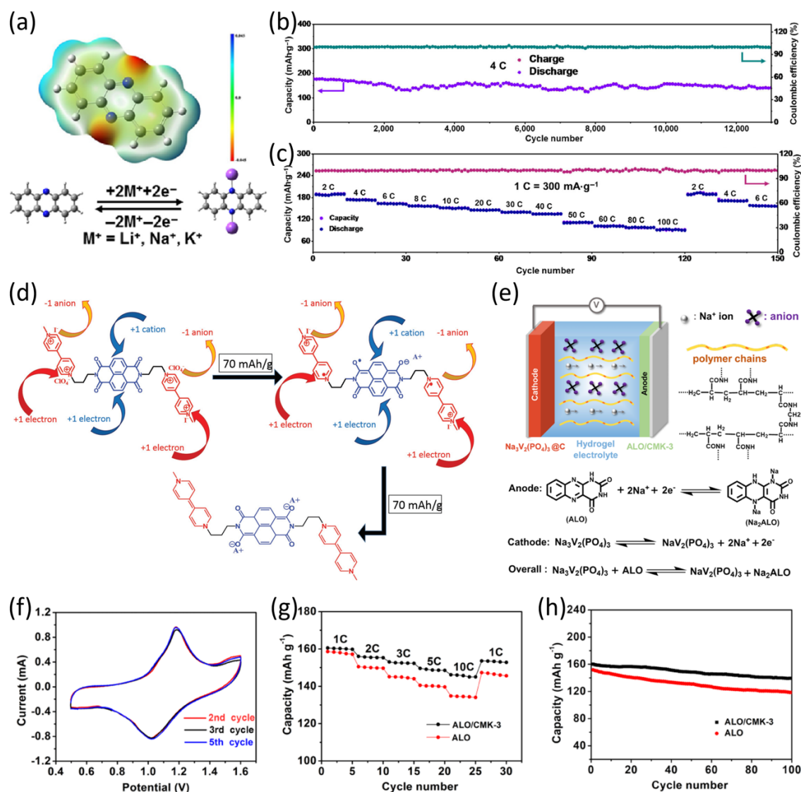
Figure 9. (a) Reaction mechanism of PNZ and molecular potential energy surface diagram. (b) Long-term cycling performance of PNZ/NMO full cell in 10M NaOH at 4 C. (c) Reversible rate
