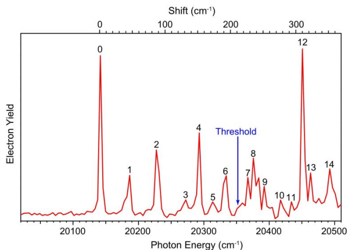
Fig. 4 The photodetachment spectrum of R\text{-TFAE}^- .
