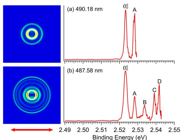
Fig. 3 Photoelectron images and spectra of R\text{-TFAE}^- at (a) 490.18 nm (2.5294 eV) and (b) 487.58 nm (2.5428 eV). The double arrow below the images indicates the laser polarization.
