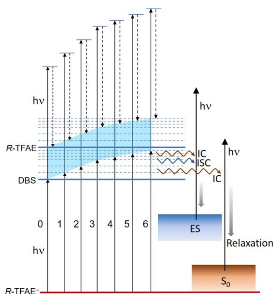
Fig. 7. Schematic energy level diagram showing the adiabatic detachment process from the bound vibrational levels of the DBS of R\text{-TFAE}^- by the second photon and the relaxation processes upon the first photon absorption. ES = excited states, IC = internal conversion, ISC = intersystem crossing.
