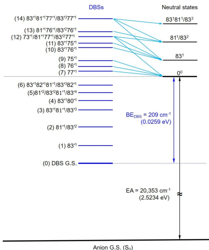
Fig. 8. The observed vibrational levels of the DBS of R -TFAE - and the autodetachment processes from the vibrational Feshbach resonances to the neutral final states. The peak numbers in Fig. 4 are given in the parentheses.
