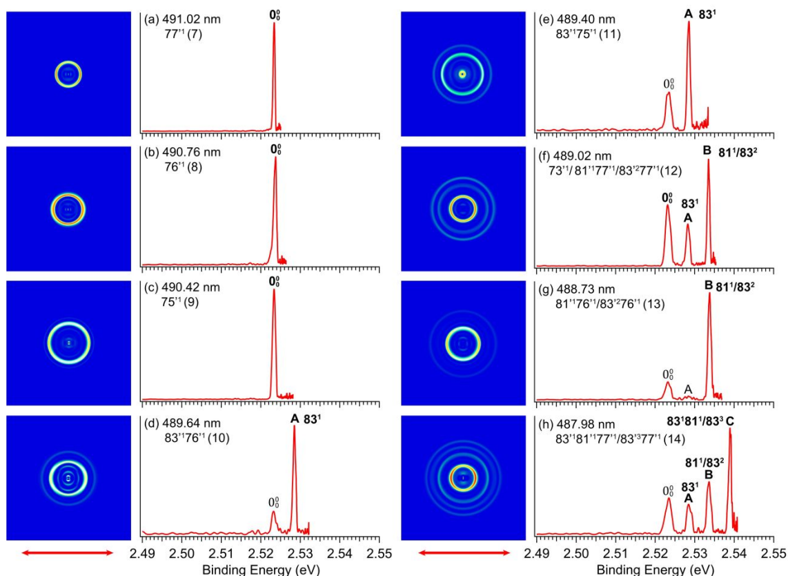
Fig. 6. Resonant photoelectron images and spectra of R\text{-TFAE}^- at (a) 491.02 nm (2.5250 eV); (b) 490.76 nm (2.5264 eV); (c) 490.42 nm (2.5281 eV); (d) 489.64 nm (2.5322 eV); (e) 489.40 nm (2.5334 eV); (f) 489.02 nm (2.5354 eV); (g) 488.73 nm (2.5369 eV); (h) 487.98 nm (2.5408 eV). The vibrational Feshbach resonances (in parenthesis) and the assignments are given. The autodetachment-enhanced vibrational peaks are labelled in bold face.
