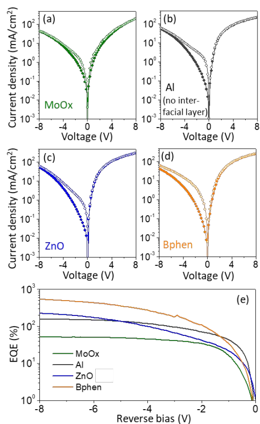
Figure 2. Current density versus applied voltage, measured in the dark (solid symbol) and under illumination (open symbol) of 4.5 mW/cm 2 from a 1050 nm LED. The interfacial layer was (a) MoOx, (b) not used and the BHJ is in direct contact with the Al electrode, (c) ZnO, and (d) Bphen. (e) External quantum efficiencies of devices with different interfacial layers.
