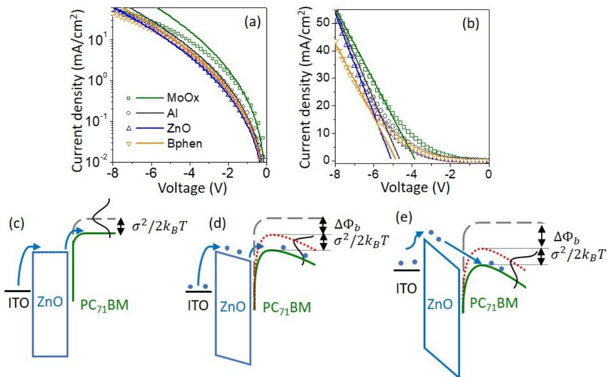
Figure 4. (a) Current densities of the devices at reverse bias in the dark, with the data represented by open symbols and the lines are fits to Equation 2a. (b) shows the data in a linear scale, and the lines are fits to Equation 2b in the high electric-field regime. The diagrams illustrate the evolving charge injection barrier at (c) flat band, (d) low electric field, and (e) high electric field. The gray dash line indicates the acceptor LUMO level, the black line represents the Gaussian distribution of energy states, the red dotted line represents the barrier lowering due to the applied electric field, and the solid green line shows the energy level available for charge injection.
