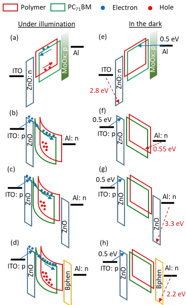
Figure 3. Energy diagrams of devices with (a, e) MoO x , (b, f) without an interfacial layer, (c, g) ZnO, and (d, h) Bphen. The devices were under reverse bias. The left column shows the photo-generated charge collection process (a) without and (b, c, d) with photomultiplication due to hole accumulation, which induced band bending that led to enhanced electron injection. The right column compares charge injection barriers in the dark.
