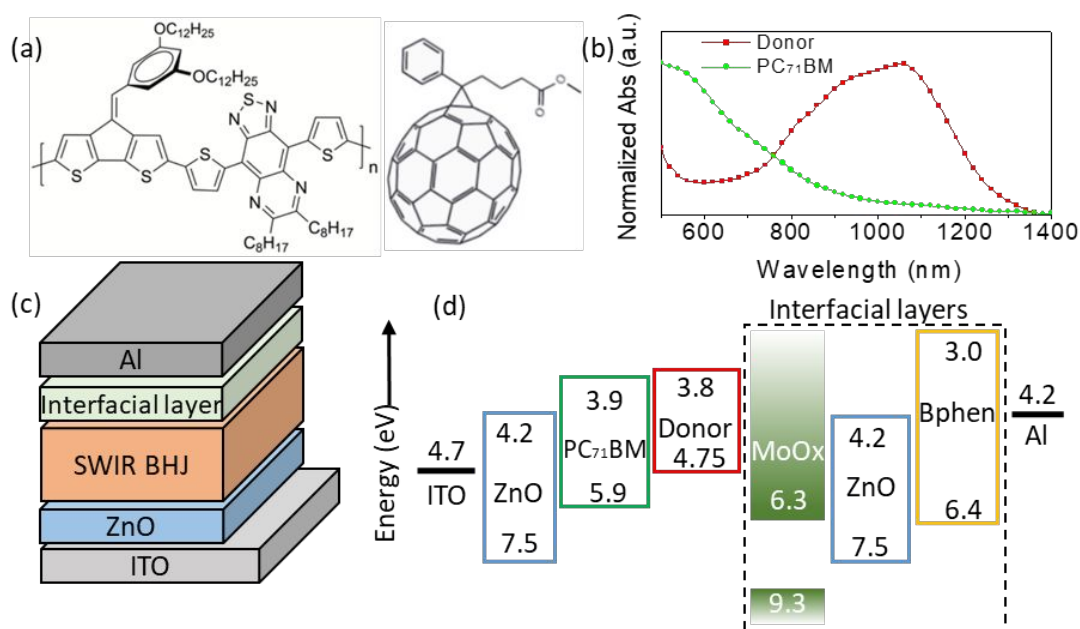
Figure 1. (a) Chemical structures of the donor and the acceptor. (b) Normalized absorbance versus wavelength. (c) A cross-sectional schematic of the device structure. (d) Energy levels of the materials used in this work.
