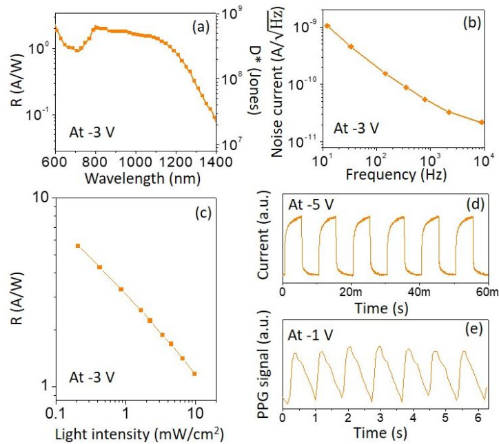
Figure 5. For the device with Bphen as the interfacial layer, (a) responsivity and specific detectivity as a function of wavelength, recorded at a frequency of 12 Hz, with the incident light intensity of 3 mW/cm 2 at 1050 nm. (b) Noise current as a function of frequency. (c) Responsivity versus light intensity from a LED emitting at the wavelength of 1050 nm. (d) Temporal response under a LED light modulated at 100 Hz. (e) Photoplethysmogram measured at a fingertip to show a person's heart rate. The LED in (d) and (e) emitted at the wavelength of 940 nm. The applied bias on the photodetector is indicated inside each panel.
