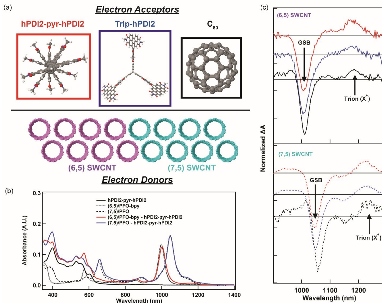
Fig. 1 (a) Molecular structures of electron acceptors, (b) Ground-state absorption spectra of SWCNT – hPDI2-pyr-hPDI2 bilayers and neat films, (black: hPDI2-pyr-hPDI2 neat film, dotted: (6,5) SWCNT neat film, dashed: (7,5) SWCNT neat film, red: (6,5) SWCNT – hPDI2-pyr-hPDI2 bilayer, blue: (7,5) SWCNT – hPDI2-pyr-hPDI2 bilayer), (c) Transient absorption spectra of SWCNT – electron acceptors at 100 ps (hPDI2-pyr-hPDI2 and Trip-hPDI2) and 300 ps (C 60 ) pump-probe delays, excited at 415 (hPDI2-pyr-hPDI2 and Trip-hPDI2) and 450 nm (C 60 ). Spectra are offset for clarity, with the ΔA=0 line provided for each spectrum.
