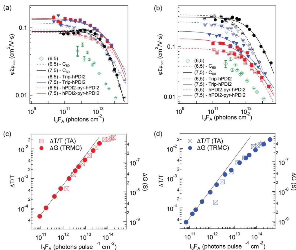
Fig. 3 (a) and (b) show the CS yield – carrier mobility product ( \phi\Sigma\mu ) vs. Absorbed Photon Fluences ( I_0F_A ) for all s-SWCNTs – electron acceptors bilayers in (a) hole transfer and (b) electron transfer. The solid lines are empirical fits to Eqn. 4, used to estimate the low-fluence limit to \phi\Sigma\mu and to interpolate \phi\Sigma\mu values appropriately for TA/TRMC comparisons. Fit is not shown for the neat (6,5) film, due to the low signal-to-noise ratio and the significant uncertainty associated with the low-fluence saturation behavior. (c) and (d) compare S_{11} \Delta T/T and TRMC \Delta G vs. I_0F_A in hole transfer at (6,5) SWCNT heterojunctions pairing with (c) hPDI2-pyr-hPDI2 and (d) Trip-PDI2.
