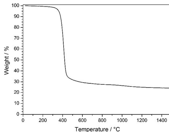
Fig. 6. TGA of stabilized PSAN colloidal crystal film after etching with HF under Argon in the temperature range of 30-1500 ^{\circ}\text{C} with a heating rate of 10 \text{K min}^{-1} .
