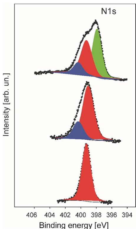
Fig. 8. The evolution of the N1s photoelectron spectrum as a function of thermal treatment of the precursor materials: original melt-sheared particle film without thermal treatment (bottom), particle film after thermal treatment at 240 °C and etching (middle), and particle films after thermal treatment at 400 °C (top). The peak areas of pyrolic-, pyridonic- and pyridinic nitrogen are shown by red, blue and green, respectively.
