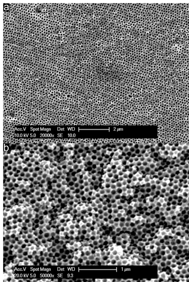
Fig. 5. SEM images of a crosslinked and stabilized PSAN colloidal crystal film after silica removal by etching with HF. a) surface topography (scalebar corresponds to 2 \mu\text{m} ) b) cross-section (scalebar corresponds to 1 \mu\text{m} ).
