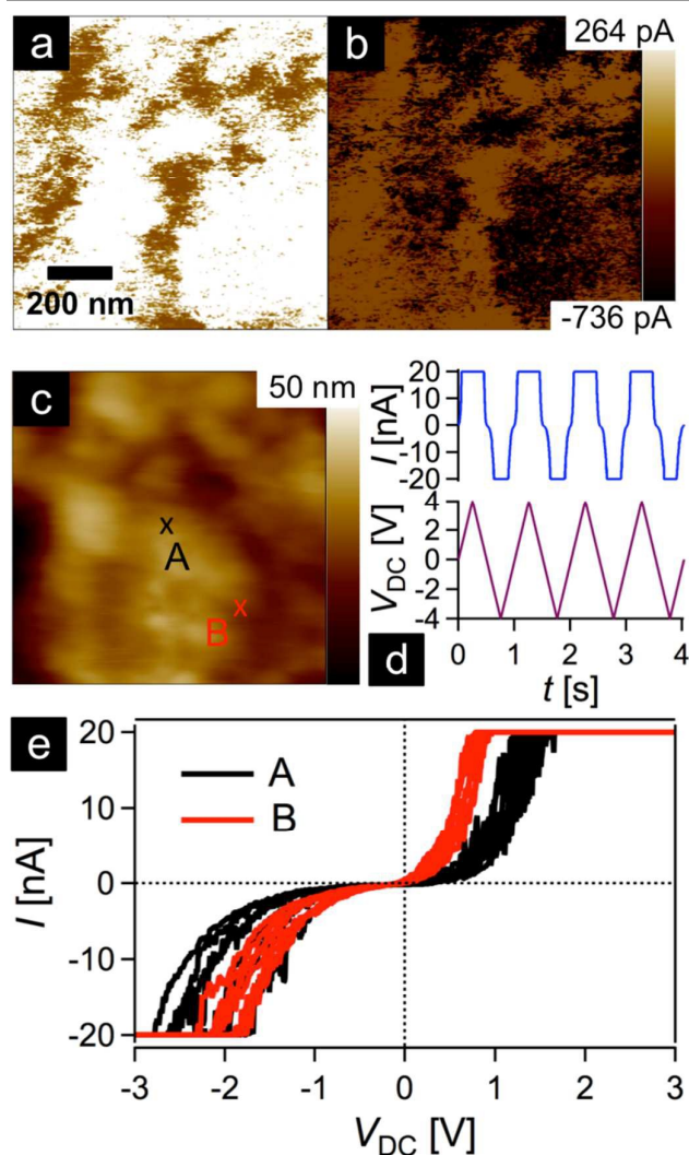
Figure 10. Conductive AFM experiment performed on a melt-shear organized particle film thermally treated at 1500 °C. (a-b) Current maps applying +1 V (a) and -1 V (b) to the sample surface, respectively, and corresponding topography image (c). (d) Current measured during four triangular voltage cycles at the position A marked in (c). (e) Current-voltage spectroscopy curves conducted at two different sample positions marked by A (black curve) and B (red curve) in the topography image of (c). Each curve consists of four consecutive cycles as shown by the current-versus-time and voltage-versus-time graphs (d).
