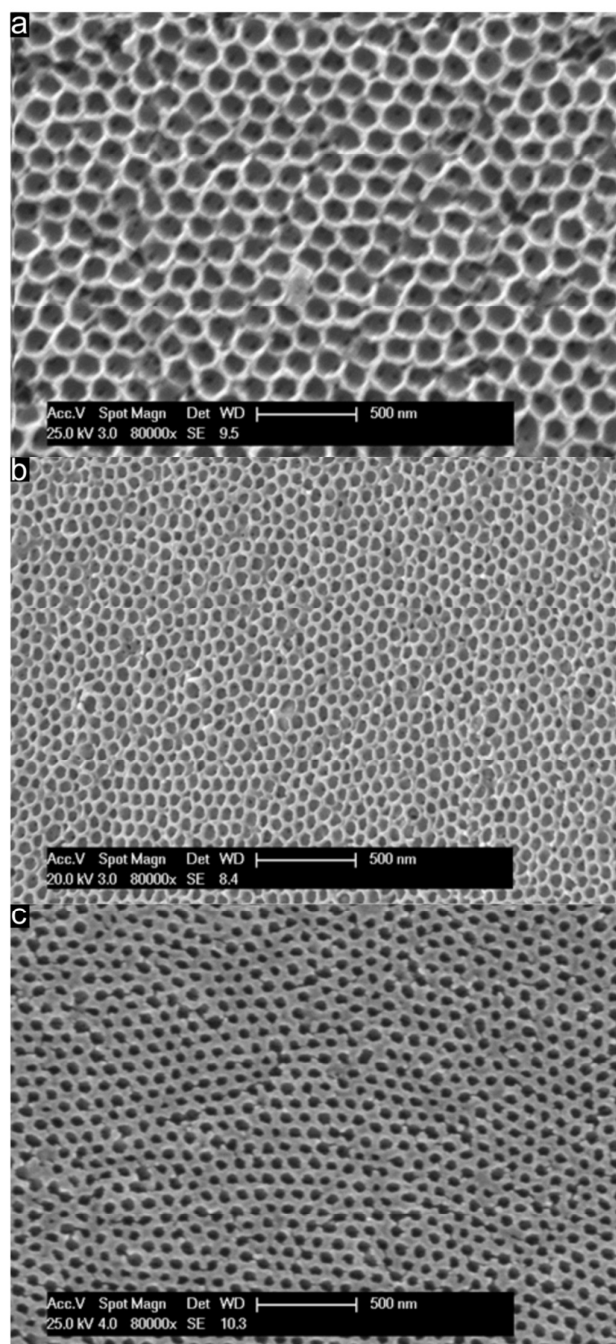
Fig. 7. SEM images of the surface of a) stabilized PSAN colloidal crystal film after thermal treatment at 240 °C and etching with HF, b) after carbonization at 400 °C and c) after graphitization at 1500 °C, showing the surface-parallel hexagonally arranged (111) plane of air voids in the matrix material.
