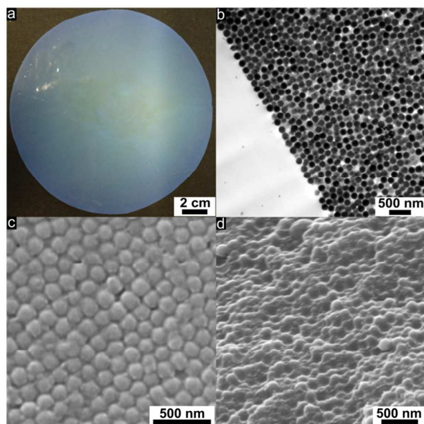
Fig. 4. a) Photograph of a silica@PSAN-based film disk (12 cm diameter) showing the strong blue reflection color. b) TEM image of an ultrathin cross-section of prepared film showing the highly-ordered the top layers and transition to disordered deeper lying polycrystalline layers. c) SEM image of the surface of silica@PSAN film after cross-linking at 240 °C showing the hexagonally arranged (111) plane of the silica spheres. d) SEM image of a cross-section of silica@PSAN film after crosslinking at 240 °C showing the silica spheres embedded in the crosslinked PSAN matrix.
