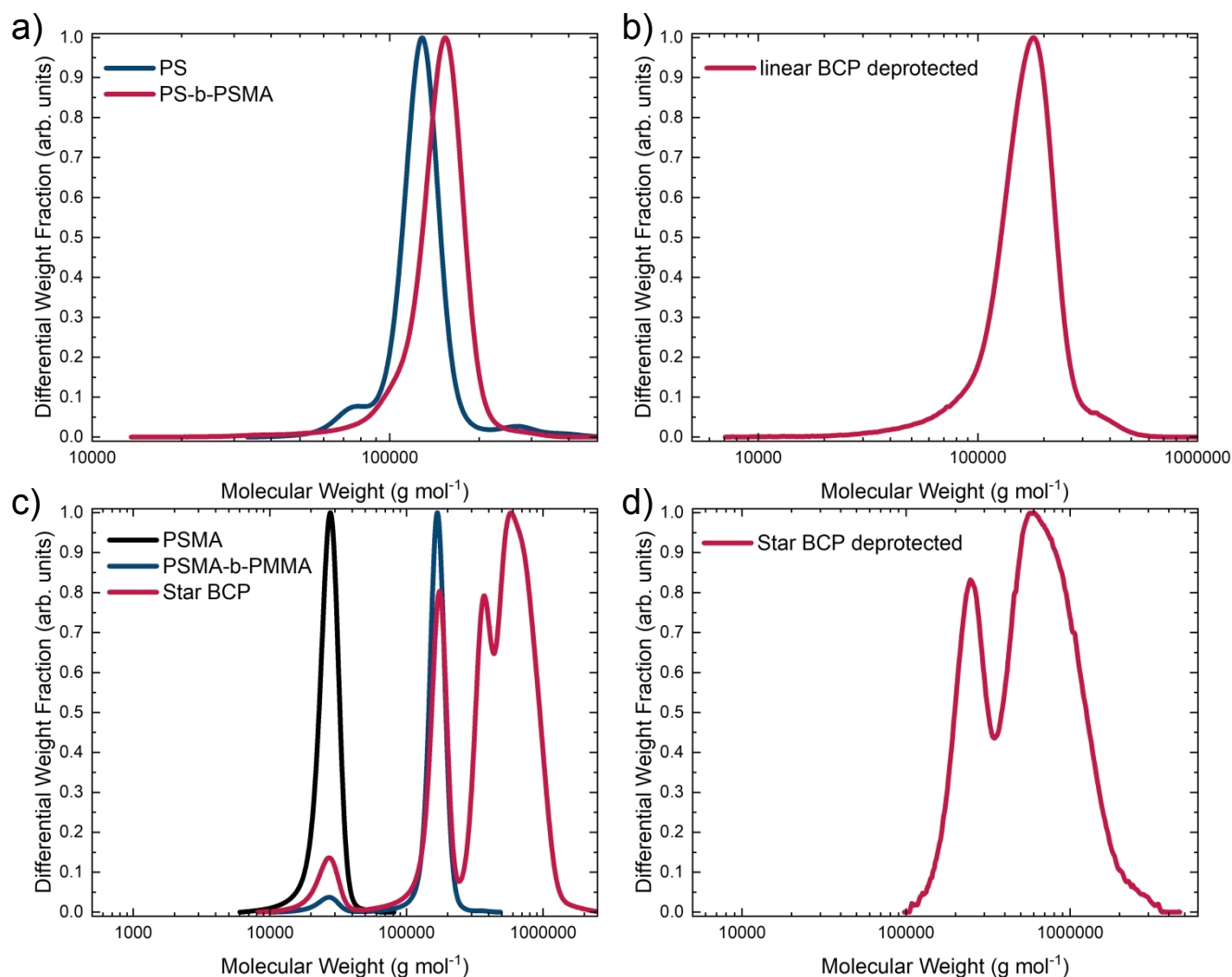
Figure 2: Compilation of SEC measurements for each step in polymer synthesis for the linear BCP (a) in THF with PS calibration, and deprotected (b) in DMF vs. PMMA calibration. The star-shaped BCP in THF vs. PS calibration is shown in (c) with its deprotected form in DMF vs. PMMA calibration (d).
