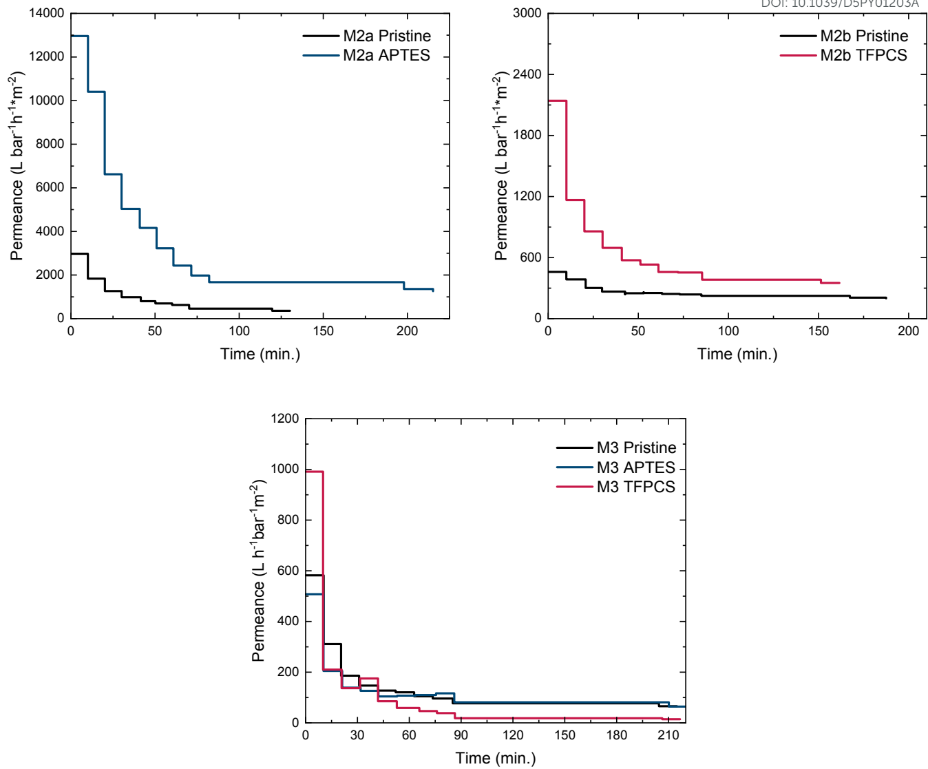
Figure 7: Water permeance measurements of membranes M2a (top left) and M2b (top right) before and after surface modification with APTES (left) and TFPCS (right). A compilation for the M3-based membranes is shown at the bottom.
