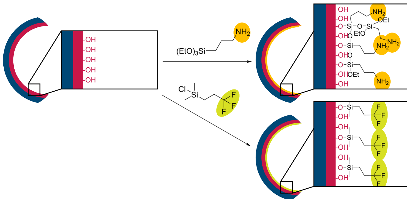
Scheme 2: Process of post-modification of a pore for APTES with possible multilayer formation (top) and TFPCS as a monolayer (bottom).
