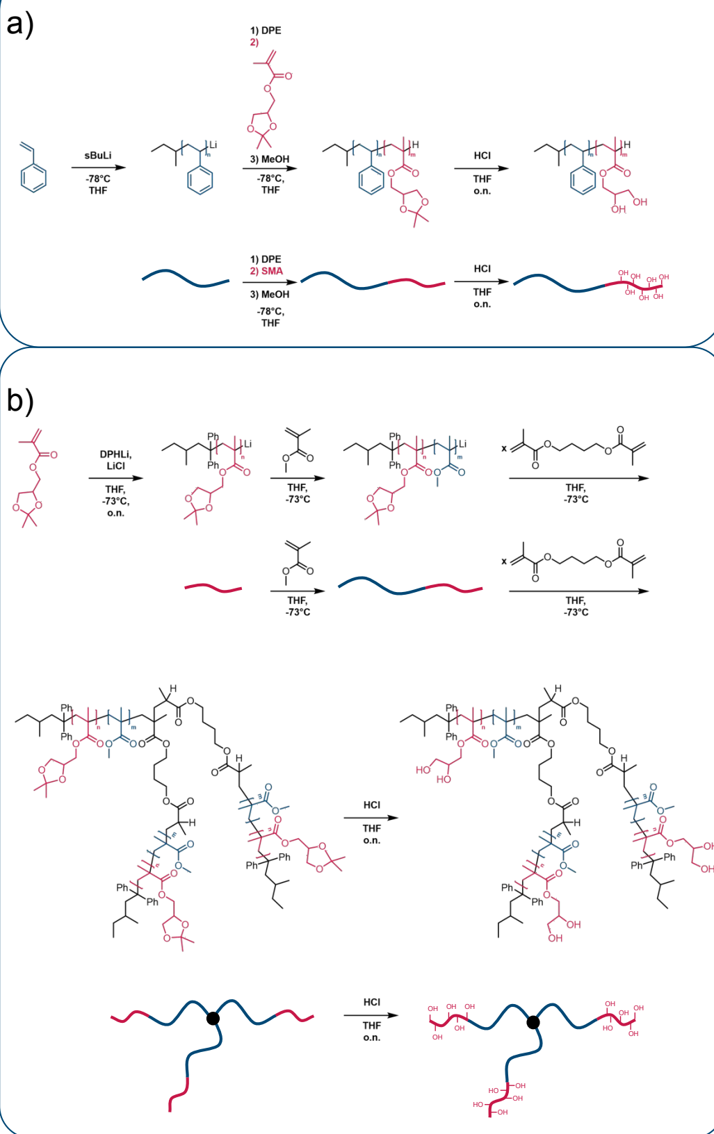
Scheme 1: Synthesis route for the linear BCP (a) and one possible star-shaped BCP (b), including the deprotection step of PSMA (red) to unveil the more hydrophilic PDHPMA block (red).
