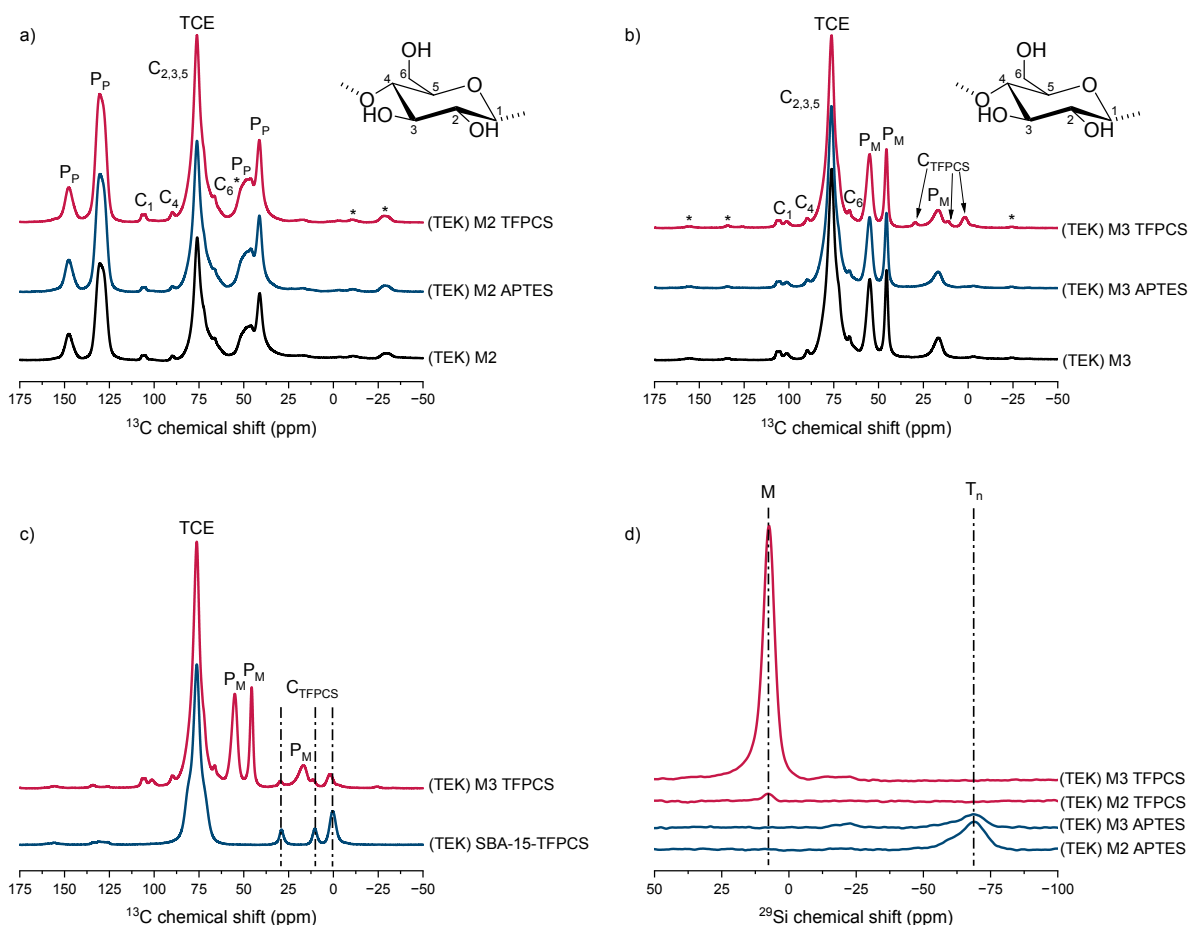
Figure 6: (a) DNP-enhanced ^1\text{H} \rightarrow ^{13}\text{C} CP MAS spectra of the unmodified membrane (Linters paper + PS- b -PDHPMA membrane (M2)), the APTES-, and the TFPCS-modified membranes measured. (b) DNP-enhanced ^1\text{H} \rightarrow ^{13}\text{C} CP MAS spectra of the unmodified membrane (Linters Paper + PMMA- b -PDHPMA membrane (M3)), the APTES-, and the TFPCS-modified membranes were measured. (c) DNP-enhanced ^1\text{H} \rightarrow ^{13}\text{C} CP MAS spectra of the TFPCS-modified SBA-15 and the TFPCS-modified membranes were measured. (d) DNP-enhanced ^1\text{H} \rightarrow ^{29}\text{Si} CP MAS spectra of the APTES- and the TFPCS-modified membranes. Note: a 15 mM TEKPol in TCE (TEK) radical-solvent system was used for sample preparations. All spectra were recorded at 8 kHz spinning. Spinning sidebands are marked with an asterisk. Signals referring to the polymer are marked with “P”.
