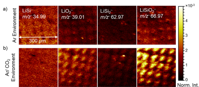
Fig. 3 Normalized SIMS 2D images in the negative ion mode of prelithiated electrodes after exposure to inert Ar gas (a) and Ar/CO 2 gas (b). The analysis area was 300 µm × 300 µm.
