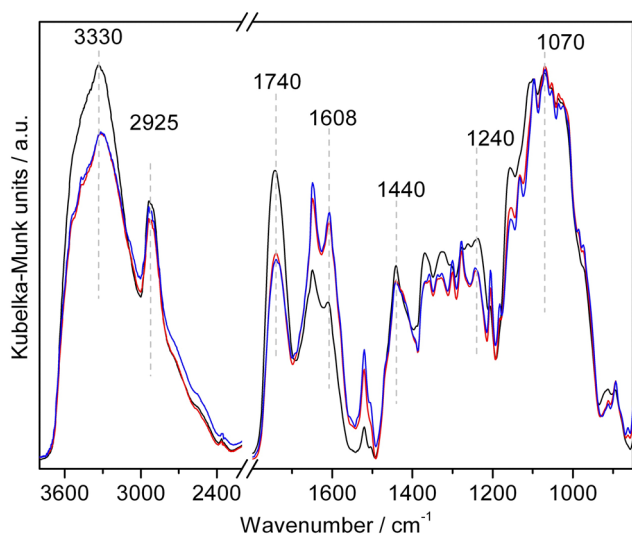
Fig. 14 DRIFT spectra of CytroCell obtained from lemon (black line), red orange (red line) and sweet orange (blue line). Spectra normalized to the band at \sim 1070 \text{ cm}^{-1} .
