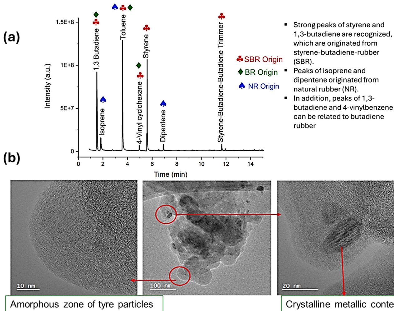
Fig. 5 (a) Pyro-GCMS furnace temperature is 600 °C; sample weight 0.175 gm; MS scan rate: m/z 29 to 600; flow rate: 1 mL \text{min}^{-1} , split ratio: 1/100; GC oven temp: 40 °C (5 min hold)-320 °C (20 °C \text{min}^{-1} , 15 min hold); (b) the HRTEM image in figure a depicts that the Tyre dusts are agglomerated. the matrix of the Tyre dust is amorphous. The metallic content (crystalline contamination) is embedded in the amorphous matrix of the Tyre dust (figure c). Authors own the analysis and images of the Tyre dust.
