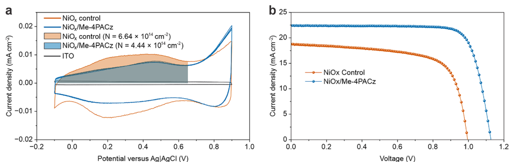
Fig. 2 CV and JV comparison between passivated and un-passivated NiO x . (a) CV for nanoparticle NiO x and NiO x /Me-4PACz. (b) JV for NiO x based PSC and NiO x /Me-4PACz based PSCs.
