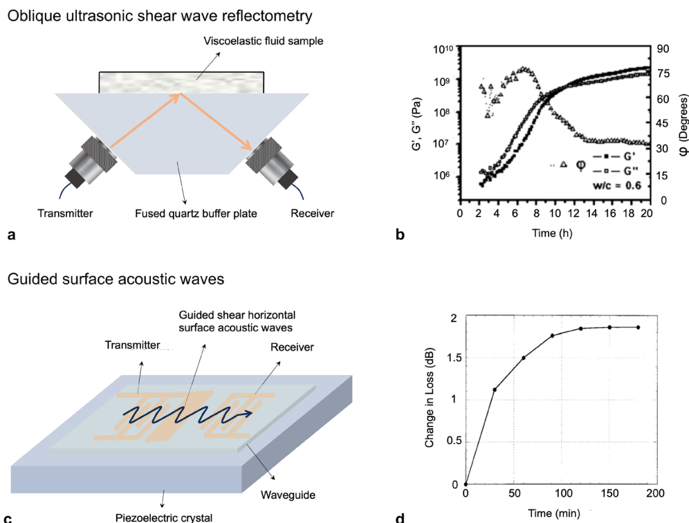
Fig. 12 Ultrasonic measurement approach for fluid viscoelasticity. (a) An illustration of obliquely incident ultrasonic shear wave reflectometry (redrawn based on ref. 234); (b) G' , G'' , and phase of shear modulus \phi as a function of elapsed time during cement paste hydration at 1 MHz for water-to-cement ratio equals to 0.6. Reproduced with permission from ref. 234. Copyright 2010, Elsevier Ltd. (c) An illustration of guided shear horizontal surface acoustic wave (SH-SAW) measurement setup (redrawn based on ref. 247); (d) changes in SH-SAW energy loss as a function of curing time for a 2 \mu\text{m} thick PMMA coating, which is an indication of the viscoelasticity change. Reproduced with permission from ref. 247. Copyright 2001, American Chemical Society.
