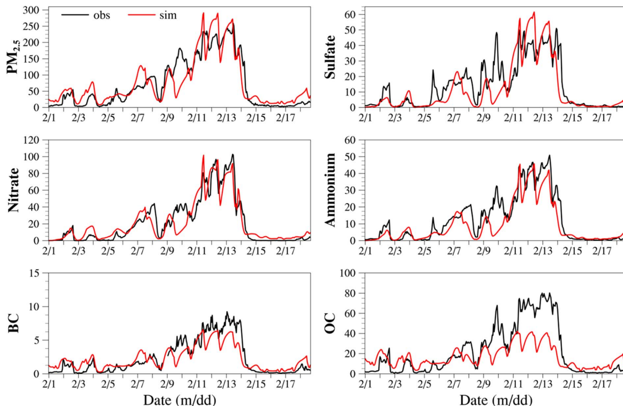
Fig. 2 The observed and model-simulated (from the M-G case) hourly concentrations of PM_{2.5} and its chemical components in Beijing from 1 to 18 February, 2020 (unit: \mu\text{g m}^{-3} ).
