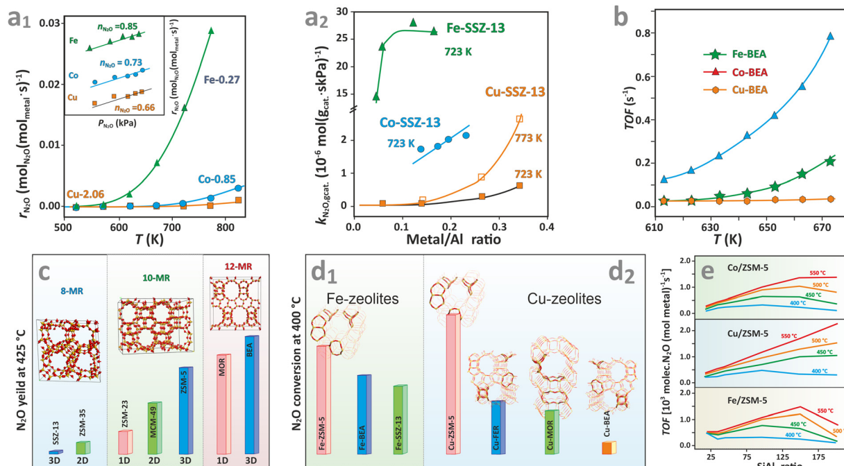
Fig. 43 Influence of the transition metal type (Co, Cu, Fe) hosted in CHA zeolites ( a_1 ) and the M/Al ratio ( a_2 ) on the \text{N}_2\text{O} decomposition performance, together with the apparent rate order ( a_1 , insert). The catalytic performance of Co, Cu, and Fe accommodated in BEA zeolites ( b ), the influence of the framework type ( c ) and ( d_1 – d_2 ), and the Si/Al ratio for Co/ZSM-5, Cu/ZSM-5, and Fe/ZSM-5 catalysts ( e ) on the \text{deN}_2\text{O} activity. Figure based on data from ref. 145, 371, 388, 390 and 391.
