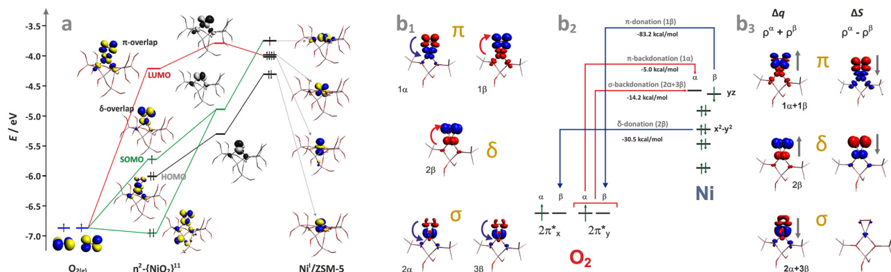
Fig. 30 Molecular orbital correlation diagram of \text{O}_2 binding to \text{Ni}^+/\text{ZSM-5} (a). The NOCV contours that describe the bonding between the dioxygen and the intrazeolite \text{Ni}^+ cation ( b_1 ), along with the corresponding diagram showing the charge and spin flow channels and the associated energies ( b_2 ), together with the orbital channels of the overall charge ( \Delta q ) and spin ( \Delta S ) flows ( b_3 ). The red and blue contours correspond to loss and gain of the electron and spin density, respectively. Adapted from ref. 64 with permission from the American Chemical Society, Copyright 2011.
