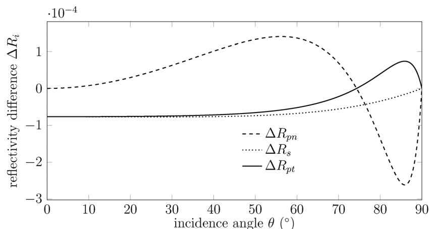
Fig. 3 Calculated reflectivity differences \Delta R_s (dotted line), \Delta R_{pt} (solid line) and \Delta R_{pn} (dashed line) plotted as a function of the incidence angle \theta for formic acid on magnetite. Calculation parameters: \nu = 1380\text{ cm}^{-1} , n_1 = 1 , k_1 = 0 , n_2 = 1.37 , 19 k_2 = 0.3 , n_3 = 3.552 , k_3 = 0 , d_2 = 0.15\text{ nm} obtained from ref. 13 and 14.
