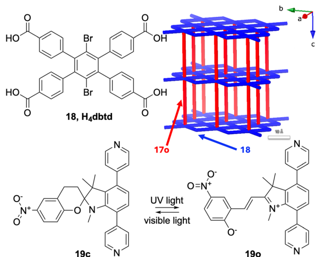
Fig. 12 Double photoswitching by incorporating the DAE 17o with the spiropyran 19c and the tetratopic carboxylate linker 18 dbtd giving various ratios of [Zn 2 ( 17o ) x ( 19c ) y (dbtd)] 2 , x + y = 1 in a paddle wheel based MOF 83 forming the 4- and 6-connected fsc -net shown in the upper right corner, drawn from the crystal structure of [Zn 2 ( 17o )(dbtd)].
