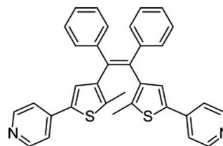
Fig. 5 The DAE (Z)-1,2-bis(2-methyl-5-(pyridin-4-yl)thiophen-3-yl)-1,2-diphenylethene 4o embedded in 19 independent crystalline materials by Benedict and co-workers where only 2 of the crystal structures suggested photochemical activity of 4, thus with C···C less than 4.2 Å and an antiparallel conformation of the methyl groups.
