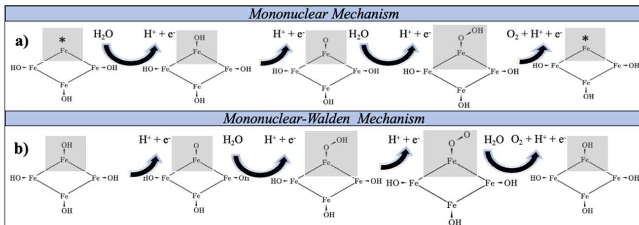
Fig. 1 Schematic representation of single-site OER mechanisms over Fe 2 O 3 (0001) based on a sketch for the \alpha -Fe 2 O 3 (0001)-4*OH surface (top view) with active sites highlighted in gray color: (a) mononuclear mechanism, starting from a partially *OH-covered surface; (b) mononuclear-Walden mechanism, starting from a fully *OH-covered surface with a concerted desorption-adsorption step.
