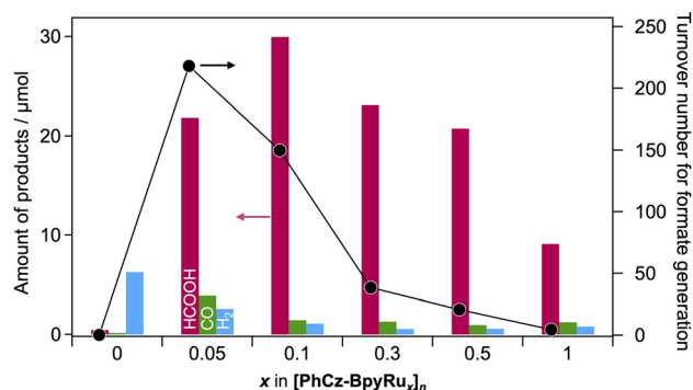
Fig. 5 Amounts of formate, CO, and H 2 formation generated over [PhCz-BpyRu x ] n (2 mg) with different loading amounts of Ru complex moiety ( x = 0, 0.05, 0.1, 0.3, 0.5, 1 ) in MeCN–TEOA (4 : 1, v/v, 2 mL) under irradiation of \lambda > 380 nm light for 6 h.
