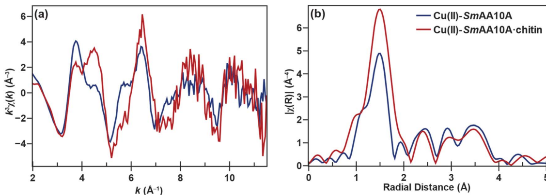
Fig. 4 (a) k^3 -weighted EXAFS and (b) FT-EXAFS of \text{SmAA10A-Cu(II)} (blue) and \text{SmAA10A}\cdot\text{Cu(II)}\cdot\text{chitin} (red). Data for the chitin-bound spectrum is derived from the 75% chitin-bound sample following subtraction.
