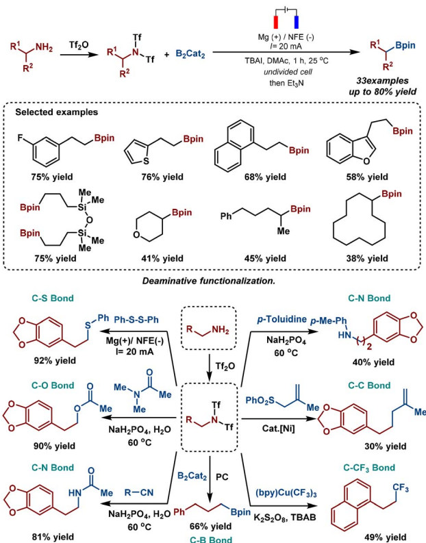
Scheme 25 Electrochemical C–B bond coupling of alkyl bistriflimides with \text{B}_2\text{Cat}_2 .
