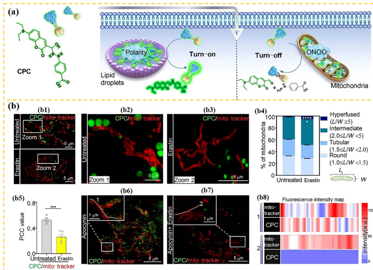
Fig. 58 (a) A schematic representation showcasing the chemical architecture of probe CPC and bimodal detection of mitochondrial \text{ONOO}^- and lipid droplet polarity. (b) Fluorescence changes of mitochondria and lipid droplets during cell iron death and SIM imaging of interactions between mitochondria and lipid droplets. (b1) SIM imaging of probes and mitochondrial commercial dye (PKMTDR) in cells induced by erastin or without erastin induction. (b2 and b3) Magnified regions of Zoom 1 and Zoom 2 in (b1). (b4) Quantitative analysis of mitochondria in or out of erastin-induced mitochondria maps. (b5) Quantitative analysis plots of mitochondrial and lipid droplet co-localization under or without erastin induction. (b6 and b7) SIM imaging of cells stained with probe CPC with PKMTDR in or out of erastin-treated apocynin-induced cells. (b8) Plots of the fluorescence intensity distribution in extended white lines 1 and 2 in (b6) and (b7). Reprinted with permission from Wiley, copyright 2024, as cited in ref. 137.
